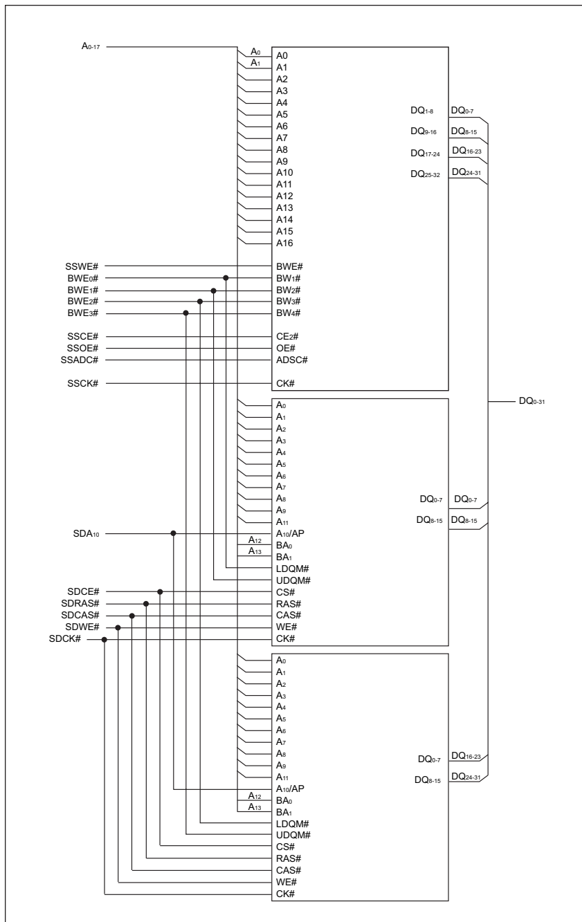
FIG. 2 BLOCK DIAGRAM
