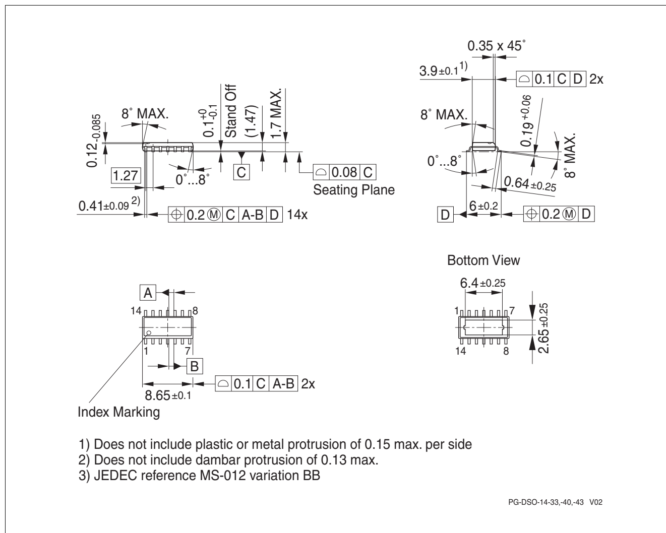
Figure 29 PG-DSO-14-40 EP (Plastic Dual Small Outline Package) (RoHS-Compliant)
