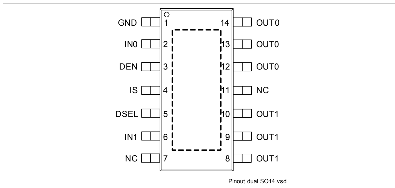
Figure 2 Pin Configuration
