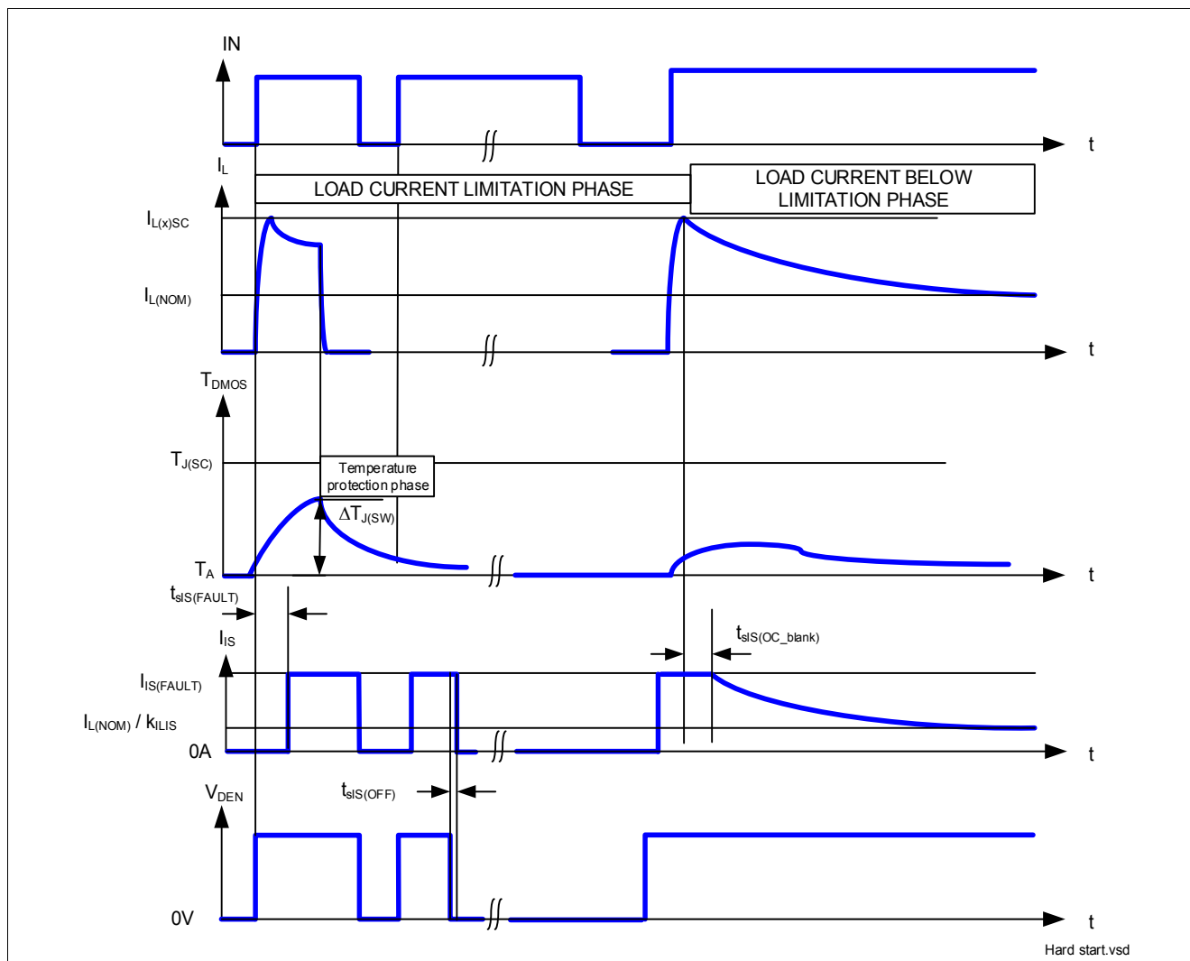
Figure 18 Overload Protection
