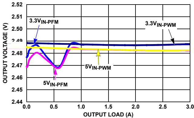
FIGURE 13. V_{OUT} REGULATION vs LOAD (1MHz, V_{OUT} = 2.5\text{V} )
