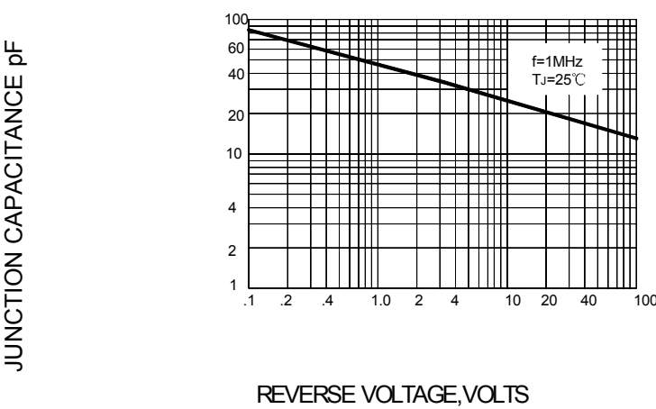
FIG.5-TYPICAL JUNCTION CAPACITANCE
