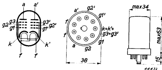
Electrode arrangement, electrode connections and max. dimensions in mm.
