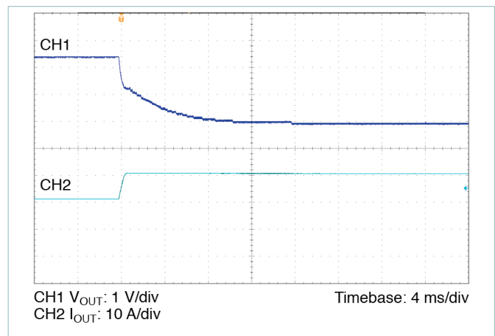
Figure 8 — 10% to 100% load transient response, V_{IN} = 300\text{ V} , nominal trim, C_{OUT\_EXT} = 220\text{ }\mu\text{F}
