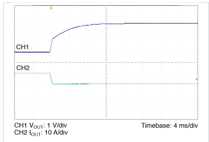
Figure 7 — 100% to 10% load transient response, V_{IN} = 300\text{ V} , nominal trim, C_{OUT\_EXT} = 220\text{ }\mu\text{F}
