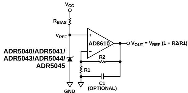
Figure 22. Adjustable Voltage Source
