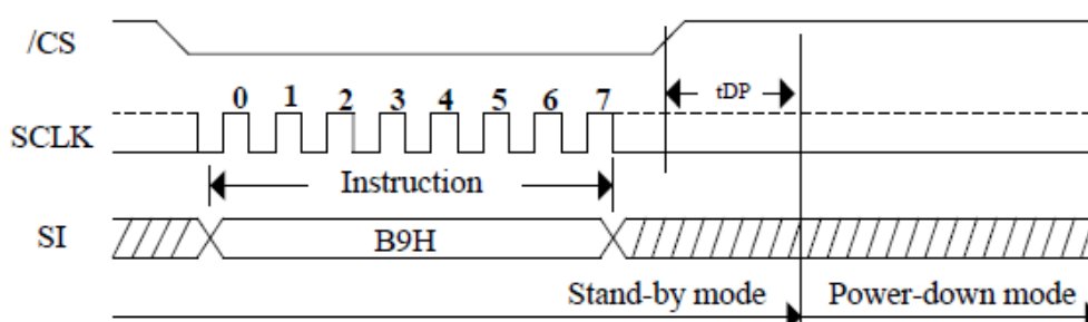
Figure 10. Deep Power-Down Sequence Diagram
