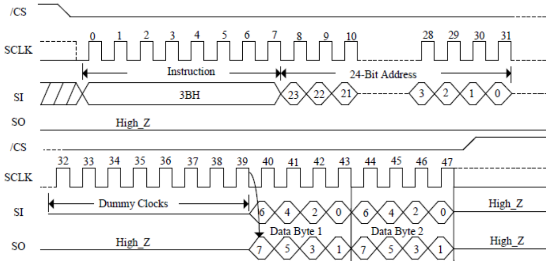
Figure 7. Dual Output Fast Read Sequence Diagram
