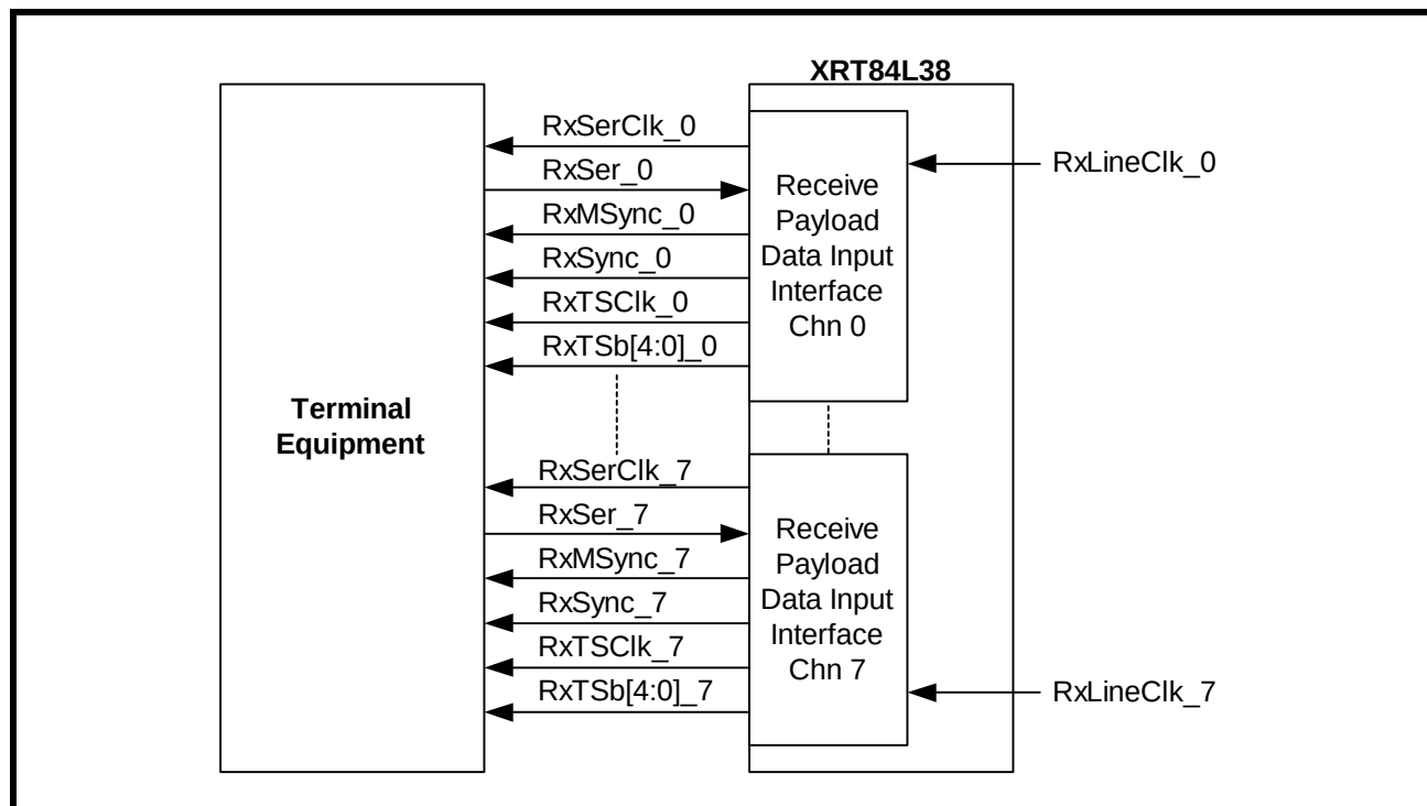
FIGURE 81. INTERFACING XRT84L38 TO LOCAL TERMINAL EQUIPMENT WITH SLIP BUFFER BYPASSED AND RECOVERED RECEIVE LINE CLOCK AS RECEIVE TIMING SOURCE
