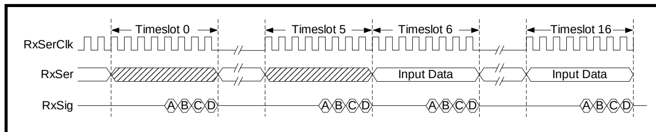
FIGURE 116. TIMING DIAGRAM OF THE RxCig_N OUTPUT PIN
