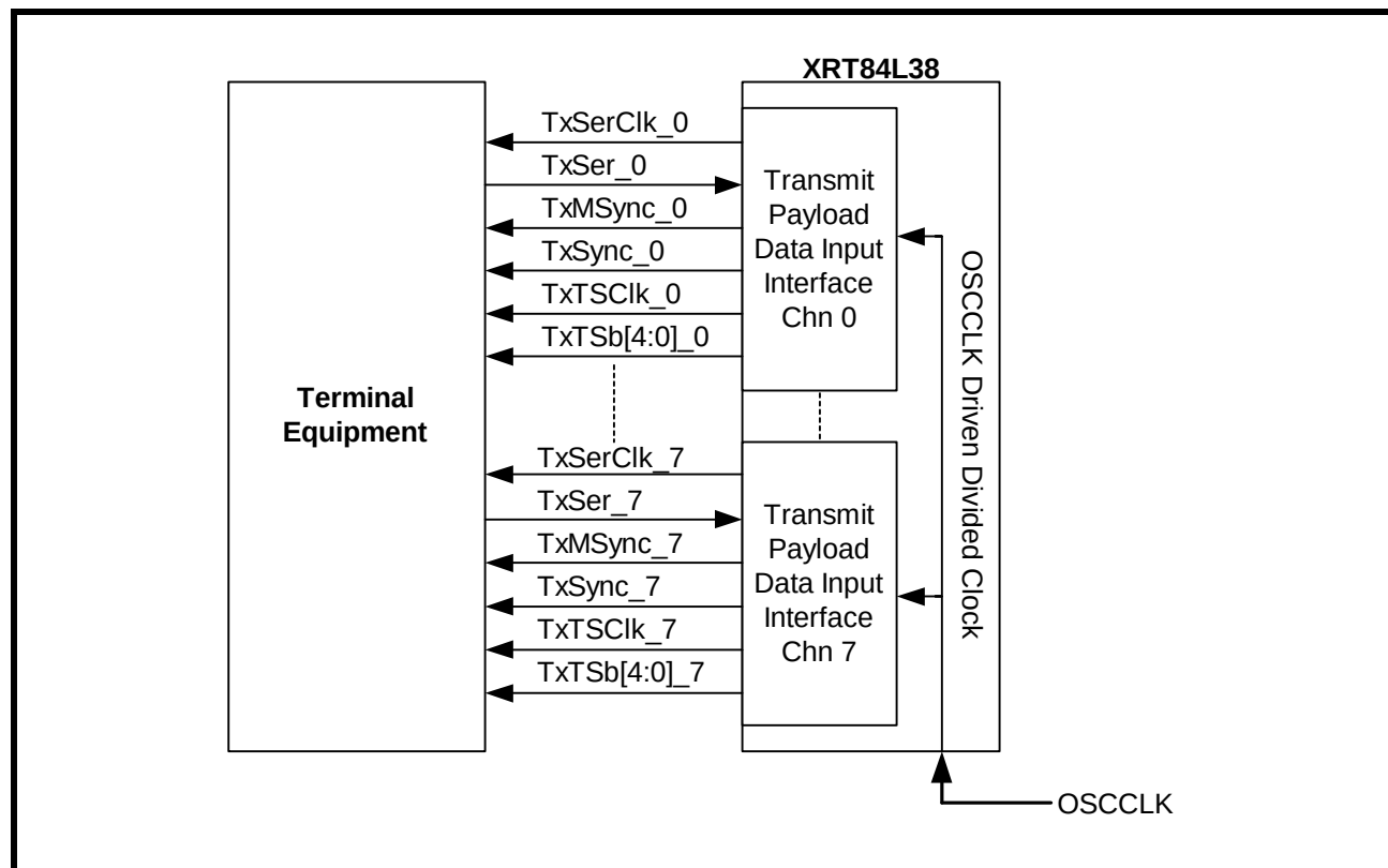
FIGURE 25. INTERFACING XRT84L38 TO THE LOCAL TERMINAL EQUIPMENT WITH THE OSCCLK DRIVEN DIVIDED CLOCK AS TRANSMIT TIMING SOURCE
