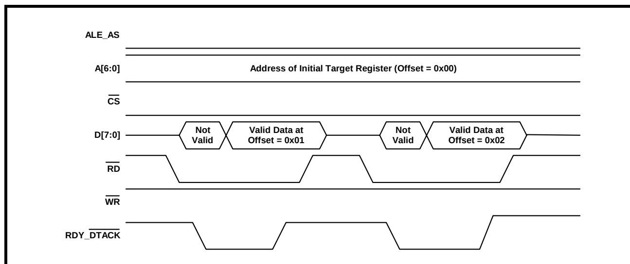
FIGURE 9. INTEL \mu\text{P} INTERFACE SIGNALS, DURING SUBSEQUENT READ OPERATIONS OF A BURST I/O CYCLE
