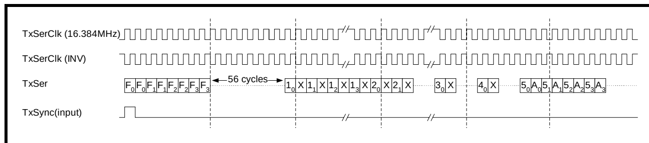
FIGURE 76. TIMING SIGNAL WHEN THE FRAMER IS RUNNING AT BIT-MULTIPLEXED 16.384MBIT/S MODE
