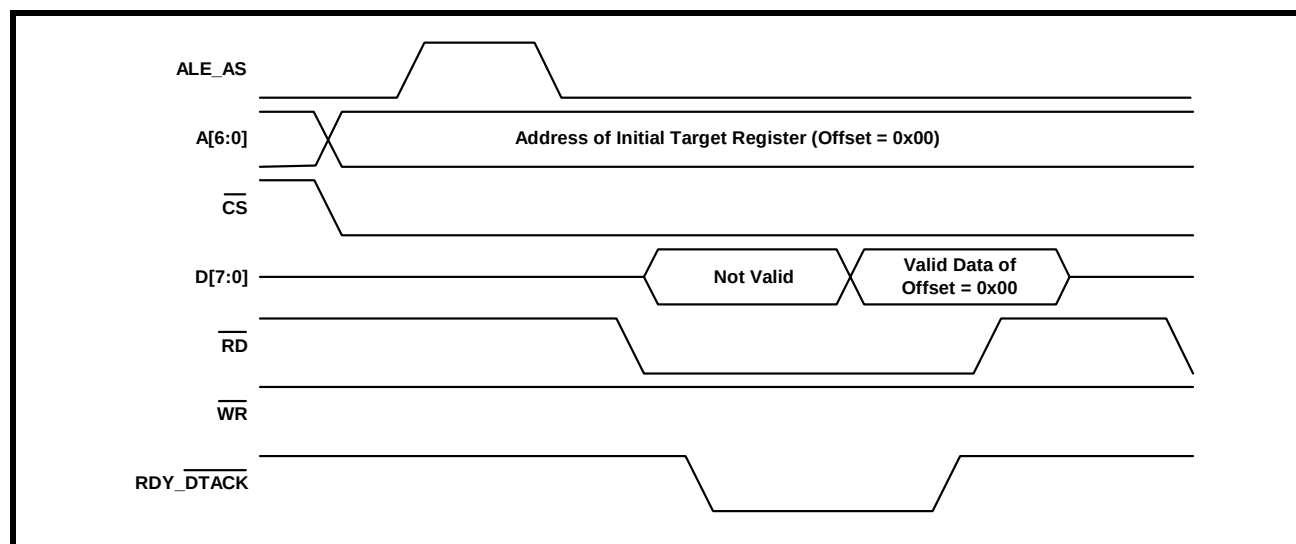
FIGURE 8. INTEL \mu\text{P} INTERFACE SIGNALS, DURING THE INITIAL READ OPERATION OF A BURST CYCLE
