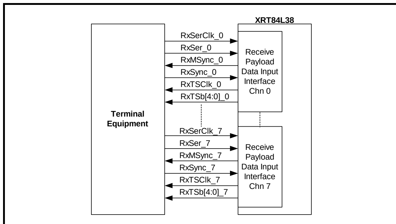
FIGURE 45. INTERFACING XRT84L38 TO LOCAL TERMINAL EQUIPMENT WITH SLIP BUFFER ENABLED OR ACTS AS FIFO
