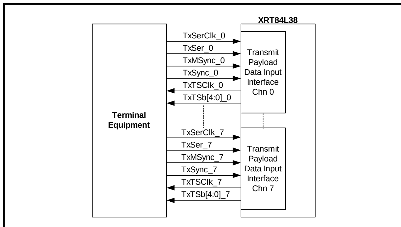
FIGURE 23. INTERFACING XRT84L38 TO LOCAL TERMINAL EQUIPMENT WITH TxSERCLK_N AS TRANSMIT TIMING SOURCE
