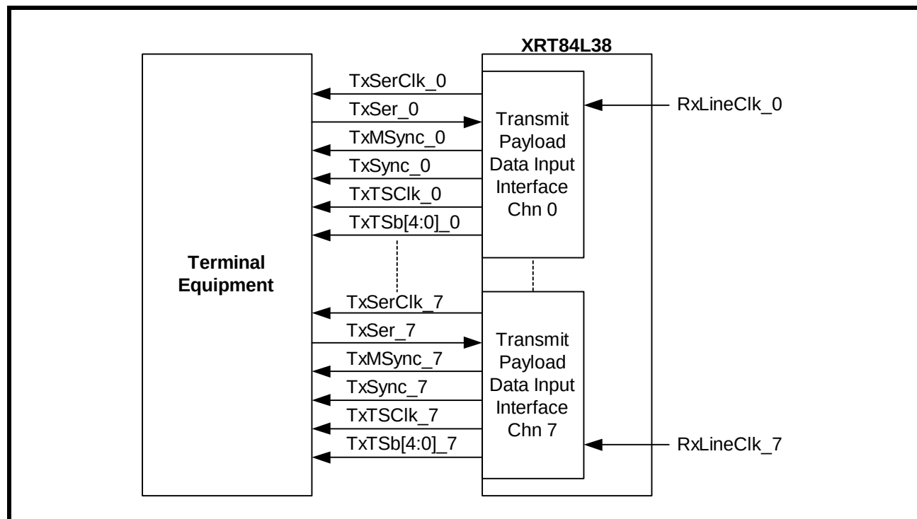
FIGURE 67. INTERFACING XRT84L38 TO LOCAL TERMINAL EQUIPMENT WITH RECOVERED RECEIVE LINE CLOCK AS TRANSMIT TIMING SOURCE
