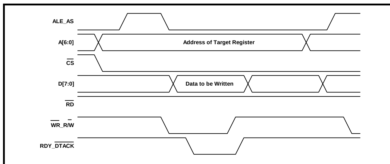
FIGURE 5. INTEL \mu\text{P} INTERFACE SIGNALS DURING PROGRAMMED I/O WRITE OPERATION
