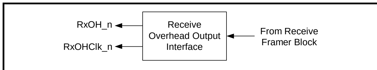
FIGURE 103. BLOCK DIAGRAM OF THE DS1 RECEIVE OVERHEAD OUTPUT INTERFACE OF XRT84L38
