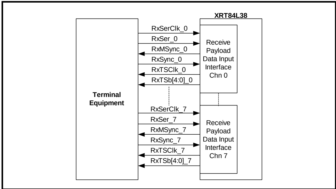
FIGURE 83. INTERFACING XRT84L38 TO LOCAL TERMINAL EQUIPMENT WITH SLIP BUFFER ENABLED OR ACTS AS FIFO
