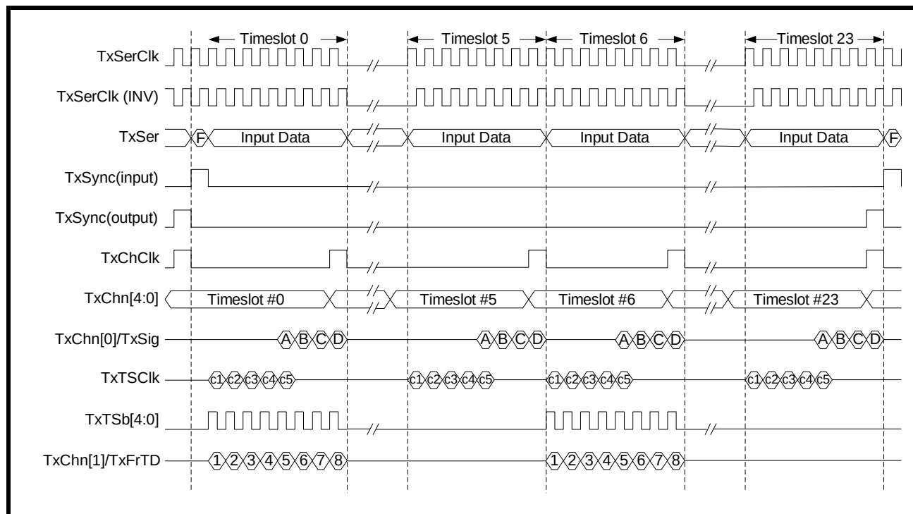
FIGURE 64. WAVEFORMS OF THE SIGNALS THAT CONNECT THE TRANSMIT PAYLOAD DATA INPUT INTERFACE BLOCK TO THE LOCAL TERMINAL EQUIPMENT WITH THE TRANSMIT SERIAL CLOCK BEING THE TIMING SOURCE OF THE TRANSMIT SECTION
