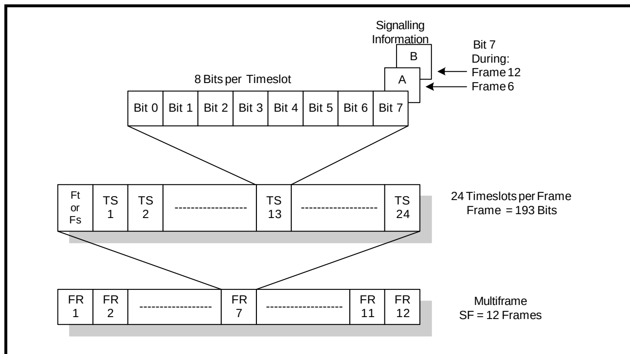
FIGURE 21. T1 SUPERFRAME PCM FORMAT
