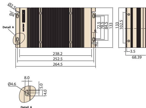
VESA mount
