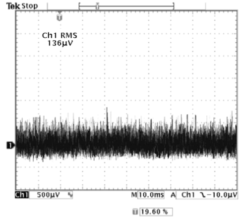
Output Noise ( I_O=0A )
