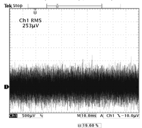
Output Noise ( I_O=300mA )
