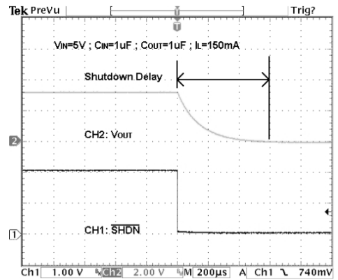
Shutdown Pin Delay
