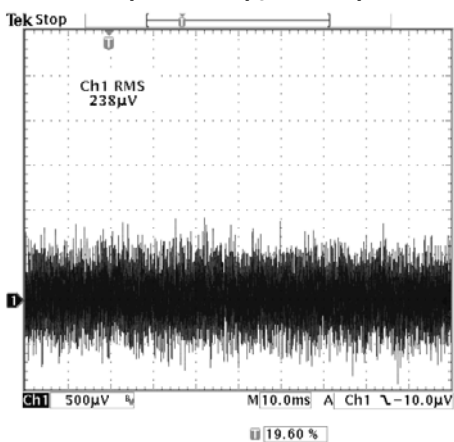
Output Noise ( I_O=150mA )
