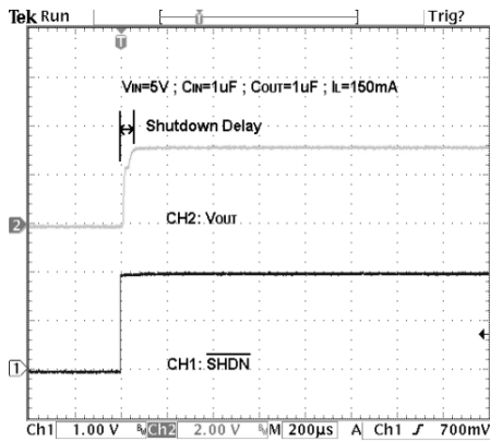
Shutdown Pin Delay
