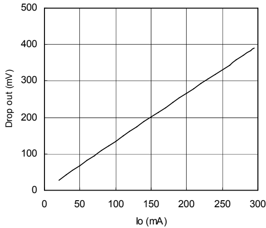
Dropout vs I_O
