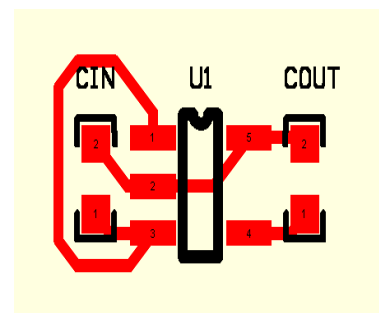
Figure 7. Fixed Mode
