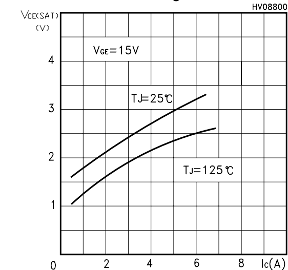
Collector-Emitter On Voltage vs Collector Current
