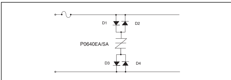
Figure 3.45 100 Base-T Protection
