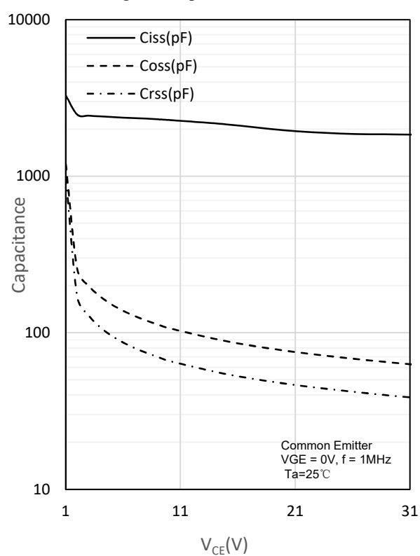
Fig. 10 Capacitance characteristics
