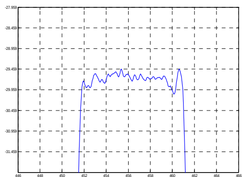
Passband Response
