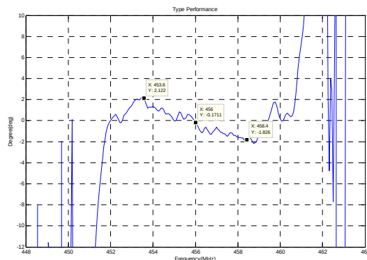
Phase Linearity(f0±2.4MHz)
