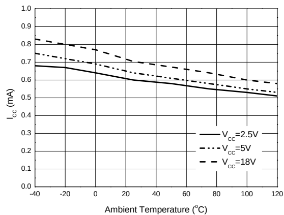
AP4306 I_{CC} vs. Ambient Temperature
