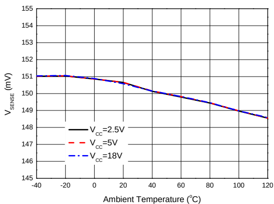
AP4306C V_{SENSE} vs. Ambient Temperature
