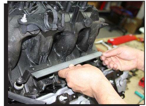
Figure 12 Straight Edge Check of Brackets.
