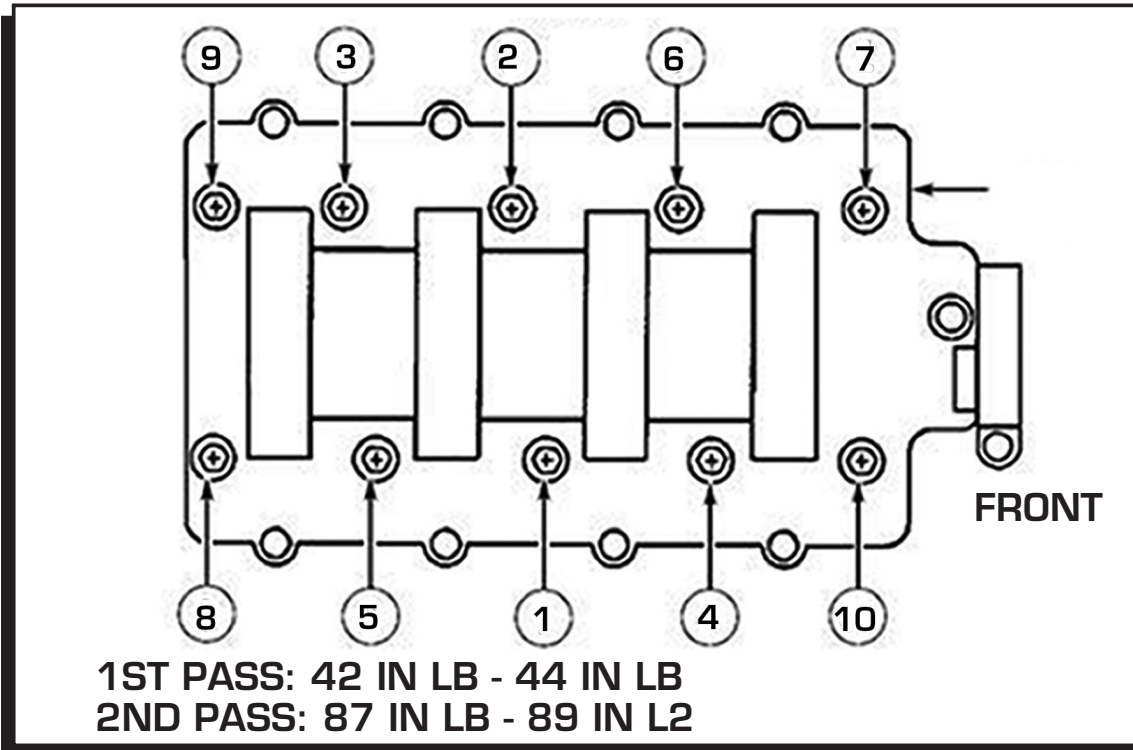
Figure 4 Intake Manifold Torque Specifications.
