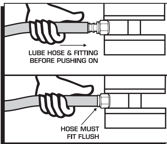
Figure 25 Installing Fuel Hose to the Push-Lock Fittings.
