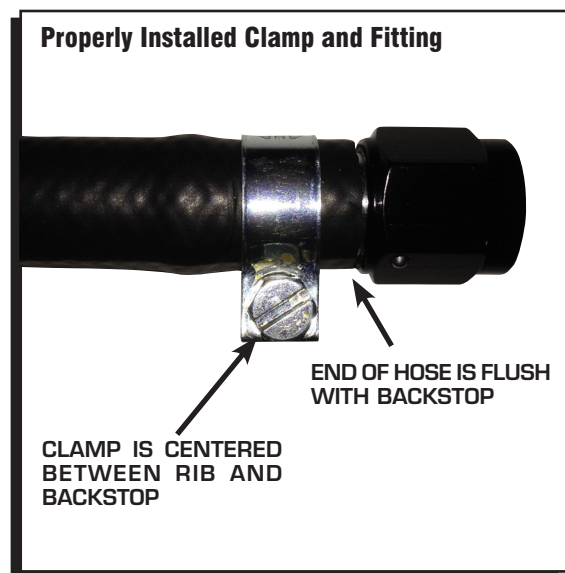
Figure 26 Installed Fitting and Clamp.
