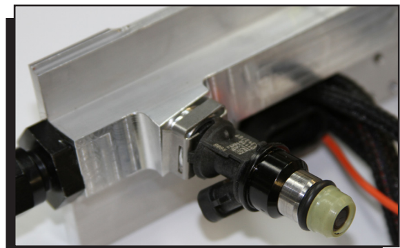
Figure 6 Injector Clips.
