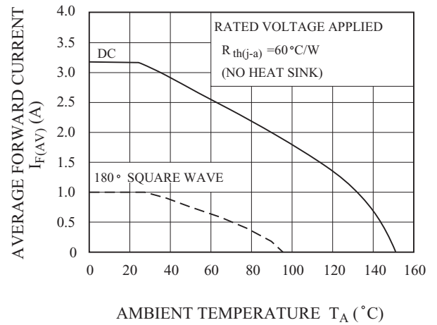
CURRENT DERATING (AMBIENT)
