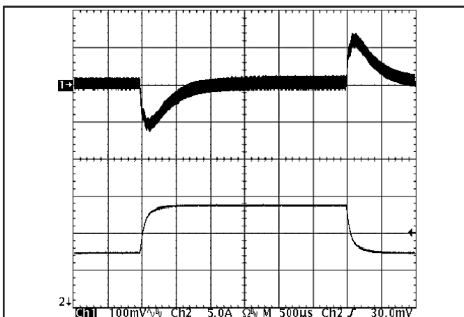
Figure 11: Output voltage response to step-change in load current (50%-75%-50% of I_{out(max)} ; dI/dt = 0.1A/\mu s ). Load cap: 10 \mu F, 100 m \Omega ESR tantalum capacitor and 1 \mu F ceramic capacitor. Ch 1: V_{out} (100mV/div), Ch 2: I_{out} (5A/div).
