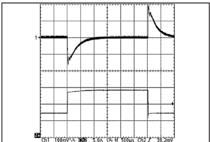
Figure 12: Output voltage response to step-change in load current (50%-75%-50% of I_{out(max)} ; dI/dt = 5A/\mu s ). Load cap: 470 \mu F, 30 m \Omega ESR tantalum capacitor and 1 \mu F ceramic cap. Ch 1: V_{out} (100mV/div), Ch 2: I_{out} (5A/div).
