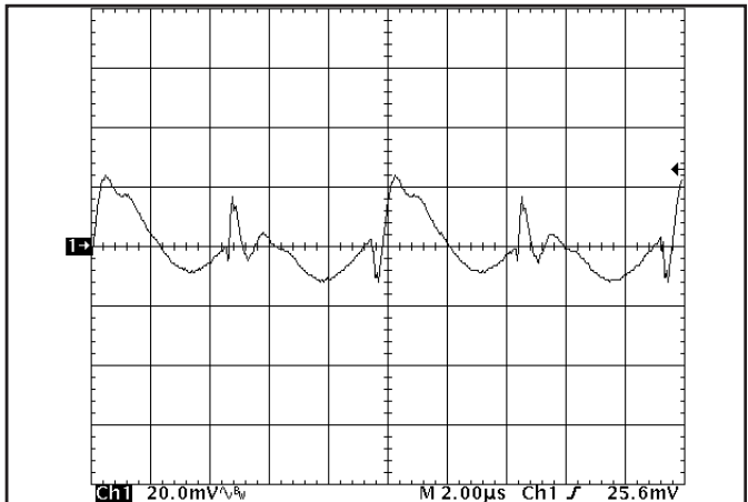
Figure 16: Output voltage ripple at nominal input voltage and rated load current (20 mV/div). Load capacitance: 1\ \mu F ceramic capacitor and 10\ \mu F tantalum capacitor. Bandwidth: 20 MHz. See Figure 13.
