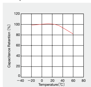
● Temperature characteristics
