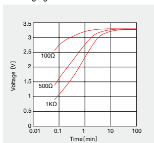
PAS414HR ● Charging characteristics
