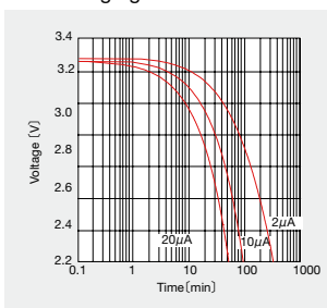
● Discharging characteristics
