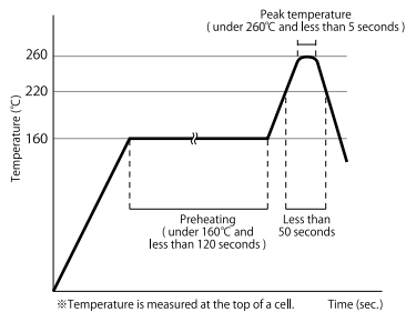
Reflow profile with lead free condition
