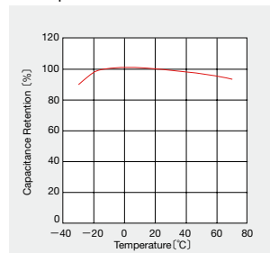
● Temperature characteristics
