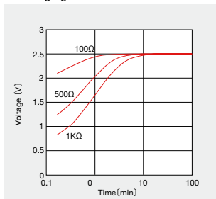
PAS414SR ● Charging characteristics
