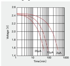
● Discharging characteristics
