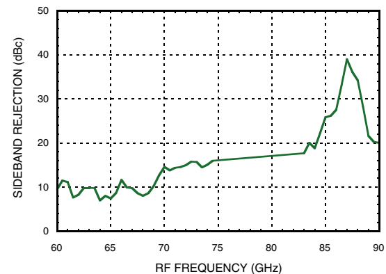
Upconverter Performance Sideband Rejection, USB
