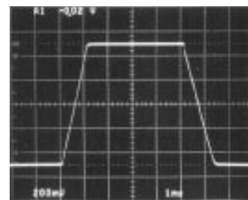
Large-Signal Response V_S = 5V, 0V
