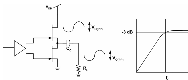
Figure 29. Single-Ended configuration and Frequency Response
