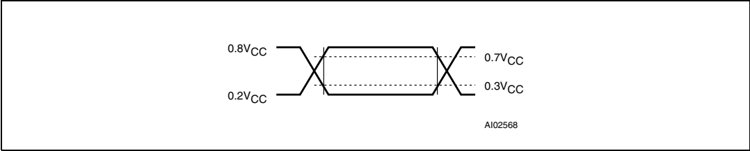
Figure 24. AC testing input/output waveforms
