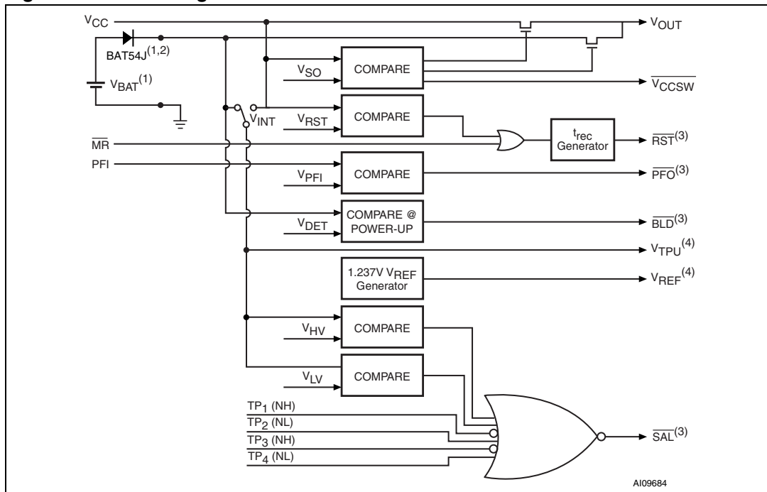
Figure 3. Block diagram
