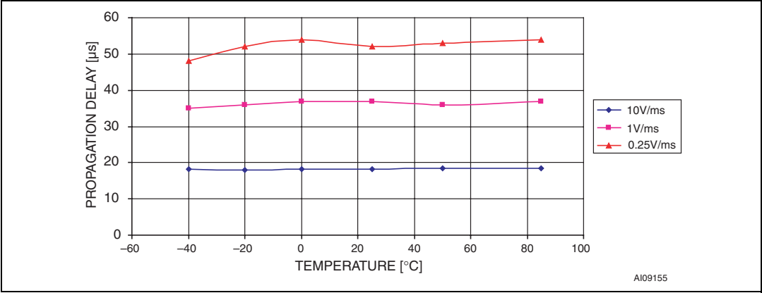
Figure 22. V_{CC} to reset propagation delay vs. temperature
