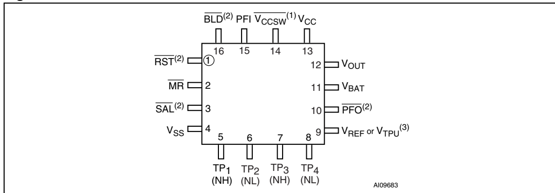
Figure 2. QFN16 connections
