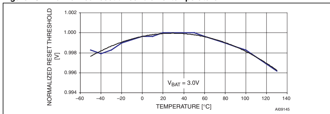
Figure 16. Normalized reset threshold vs. temperature
