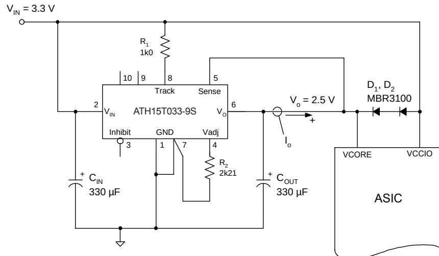
Figure 3.8; Application Circuit Demonstrating Pre-Bias Startup
