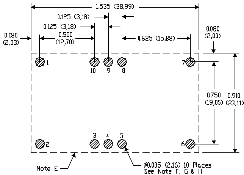
PC LAYOUT
