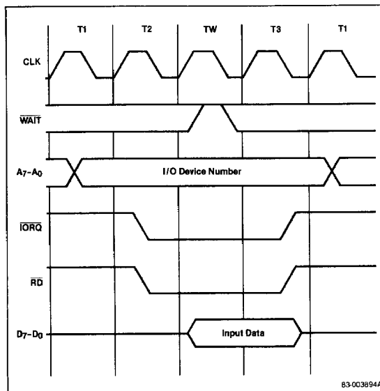
Figure 6. I/O Read Cycle
