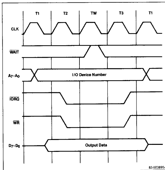
Figure 7. I/O Write Cycle
