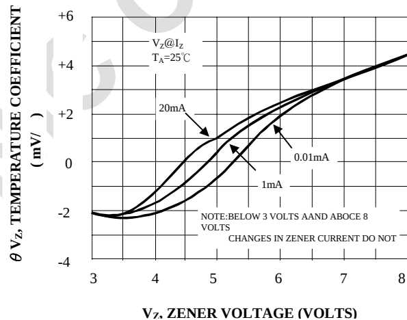
Figure 4. Effect of Zener Current
