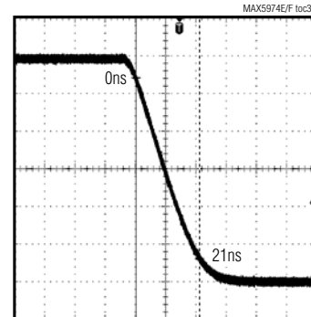
AUXDRV 90% TO 10% FALL TIME
