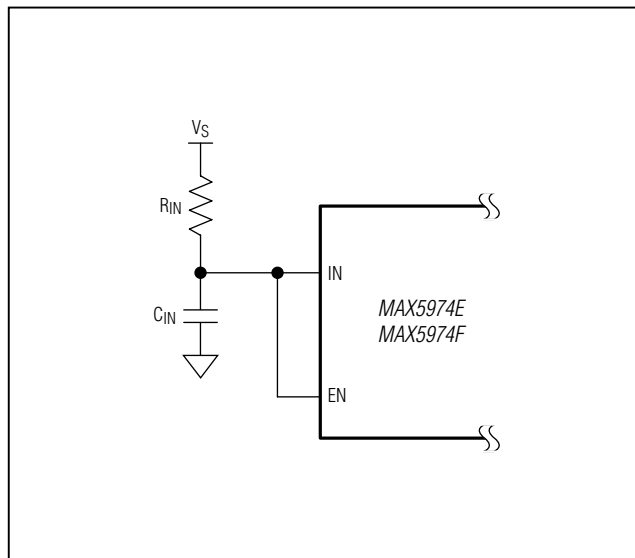
Figure 4. Always-On Operation
