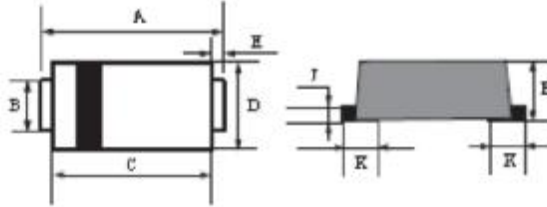
SOD123-FL
