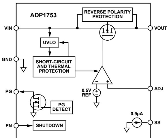
Figure 25. ADP1753 Internal Block Diagram
