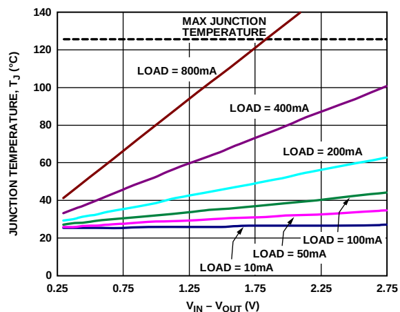
Figure 37. 500 mm 2 of PCB Copper, T_A = 25^\circ\text{C} , LFCSP
