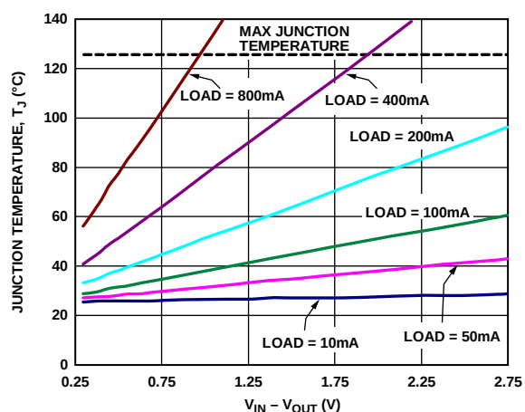
Figure 38. 0 mm 2 of PCB Copper, T_A = 25^\circ\text{C} , LFCSP
