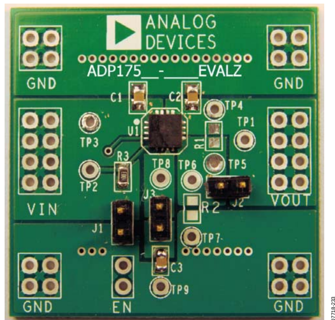
Figure 46. Evaluation Board
