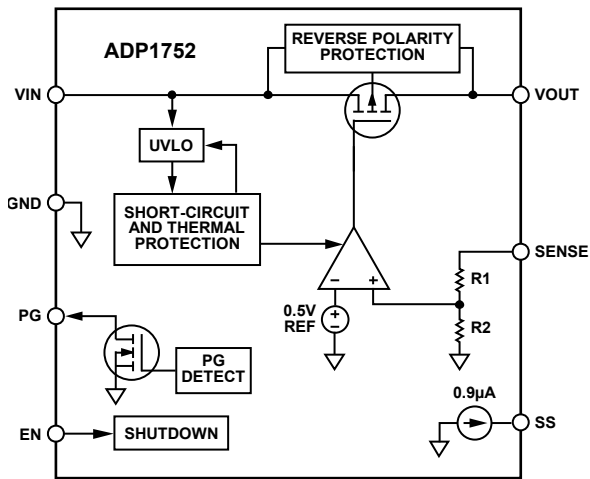
Figure 24. ADP1752 Internal Block Diagram
