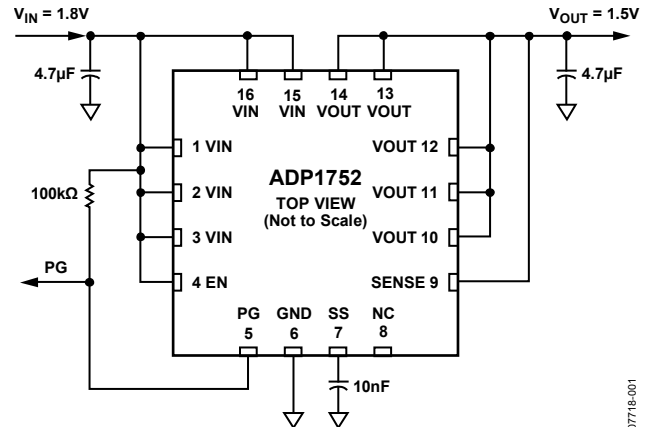
Figure 1. ADP1752 with Fixed Output Voltage, 1.5 V
