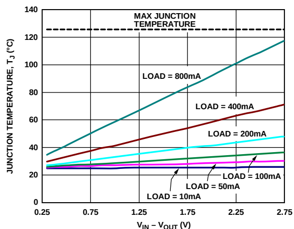
Figure 36. 6400 mm 2 of PCB Copper, T_A = 25^\circ\text{C} , LFCSP
