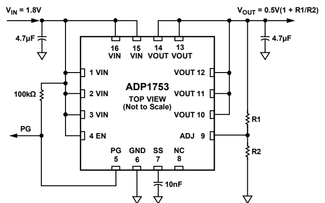
Figure 2. ADP1753 with Adjustable Output Voltage, 0.75 V to 3.3 V
