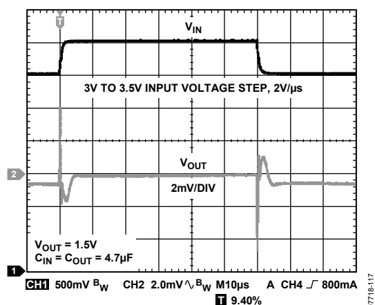
Figure 17. Line Transient Response, Load Current = 800 mA
