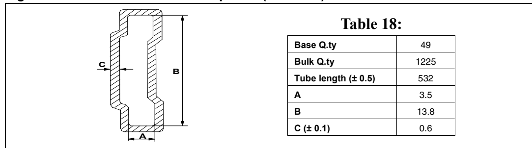
Figure 36. PowerSSO-24 tube shipment (no suffix)
