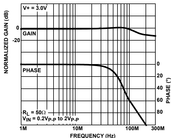
FIGURE 21. FREQUENCY RESPONSE
