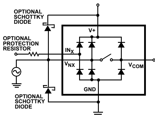
FIGURE 8. OVERVOLTAGE PROTECTION
