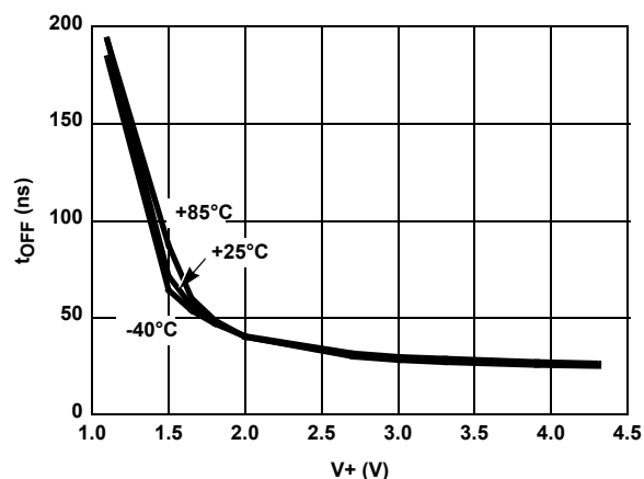
FIGURE 20. TURN-OFF TIME vs SUPPLY VOLTAGE
