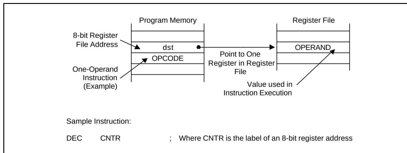
Figure 3-1. Register Addressing
