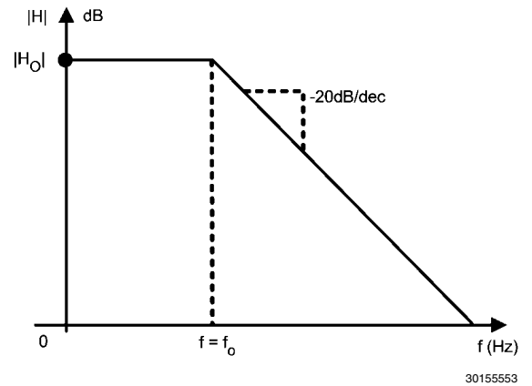
FIGURE 4. Lowpass Filter Transfer Function
