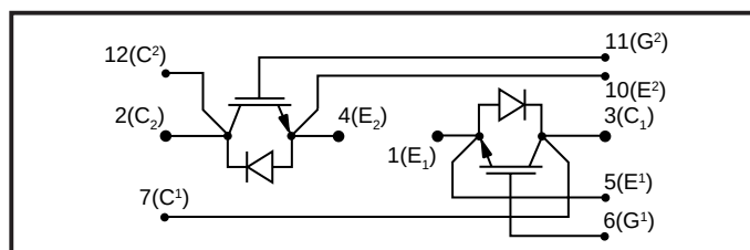
Fig.2 Dual switch circuit diagram
