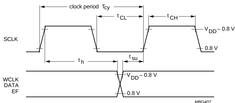
Fig.33 I 2 S-bus timing diagram.
