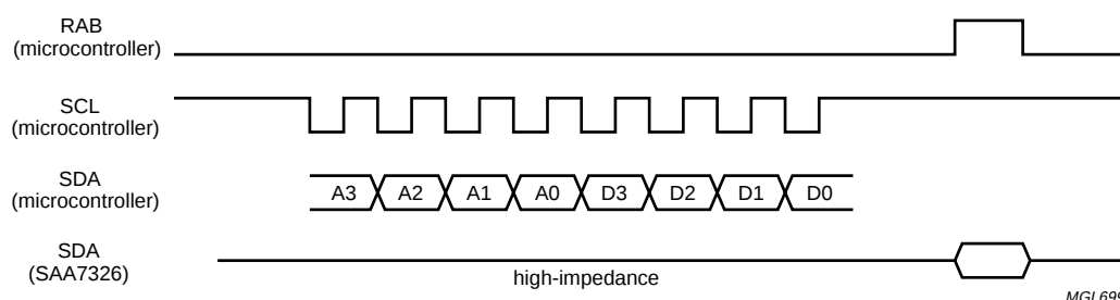
Fig.23 Microcontroller write protocol for registers 0 to F.
