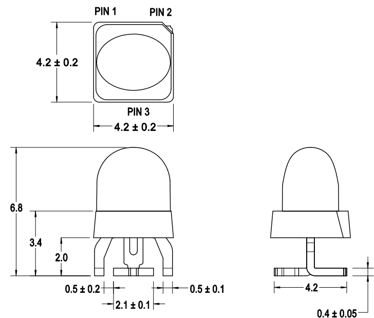
Figure 1: Package Drawing
