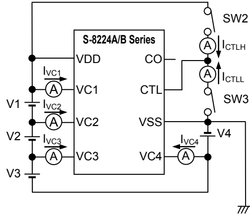
Figure 8 Test Circuit 4
