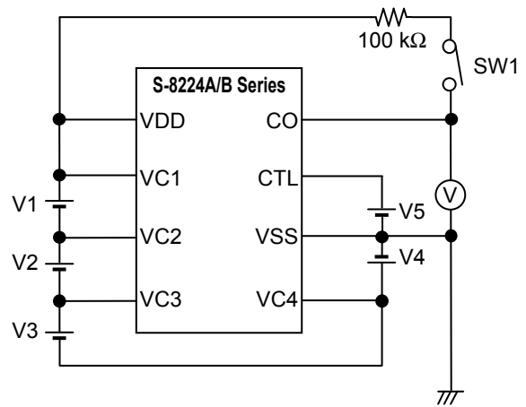
Figure 6 Test Circuit 2
