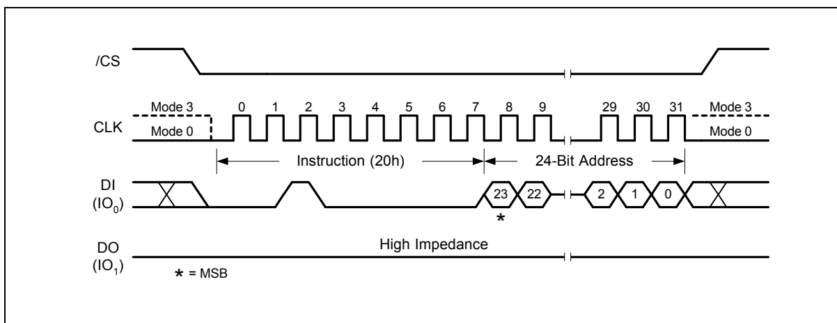
Figure 15. Sector Erase Instruction Sequence Diagram
