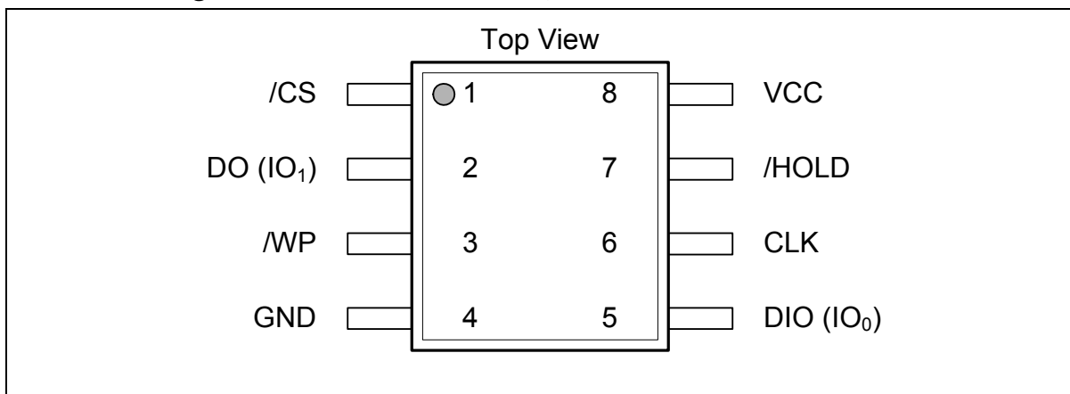
Figure 1a. W25X40BL Pin Assignments, 8-pin SOIC 150 / 208-mil, VSOP 150-mil (Package Code SN, SS & SV)
