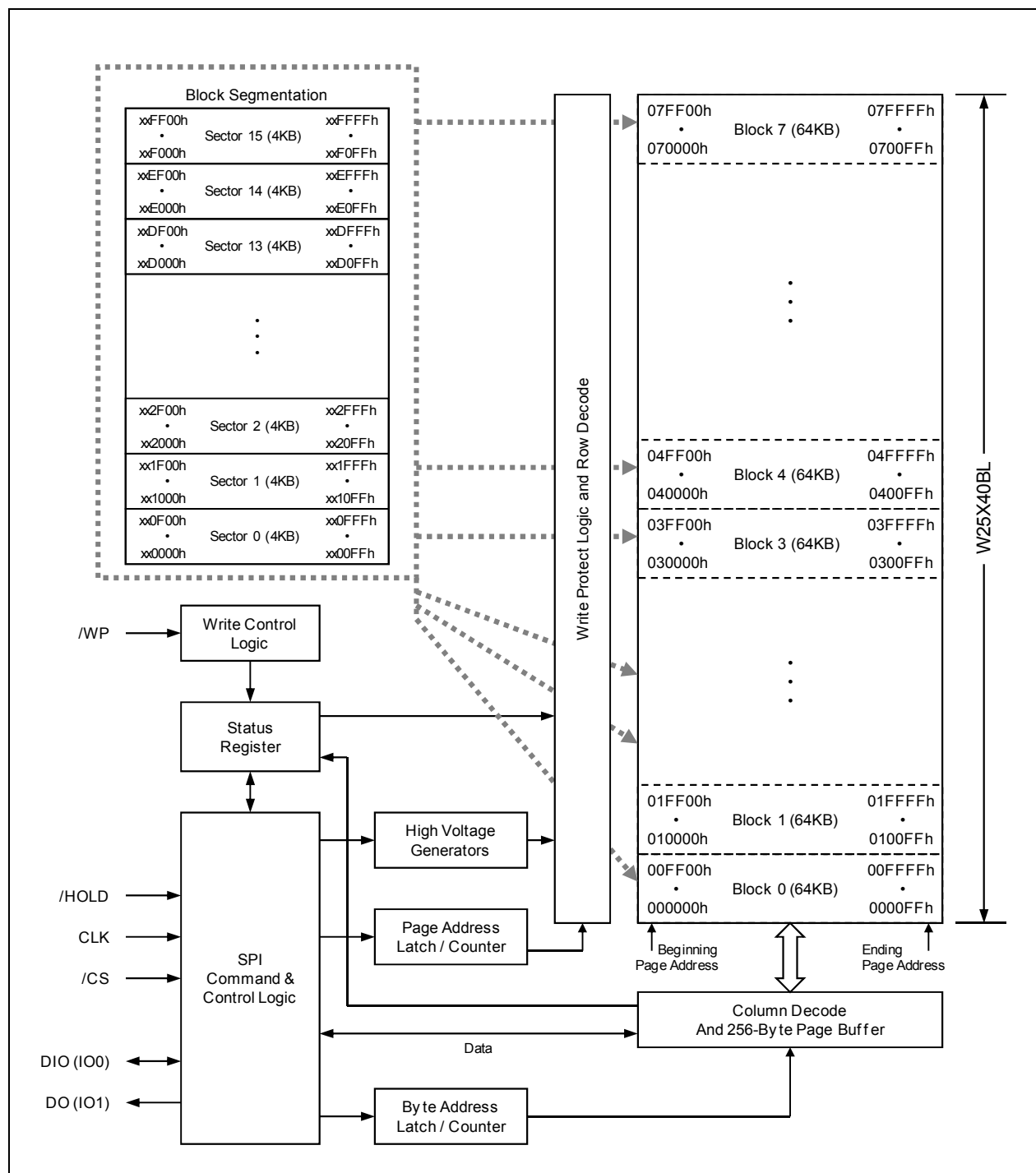
Figure 2. W25X40BL Block Diagram
