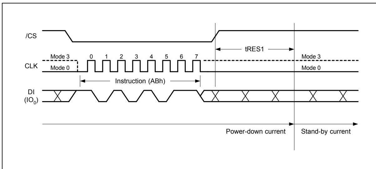
Figure 20. Release Power-down Instruction Sequence
