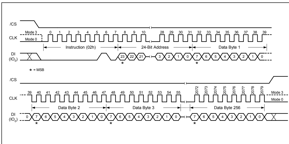
Figure 14. Page Program Instruction Sequence Diagram
