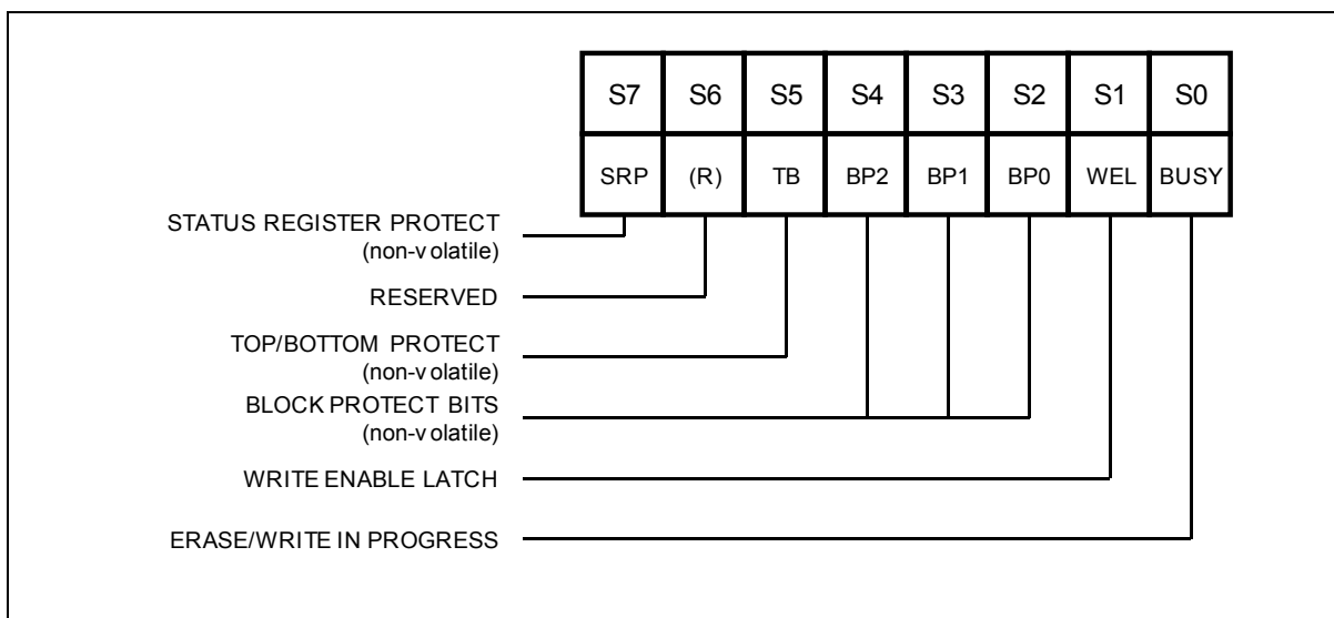
Figure 3. Status Register Bit Locations
