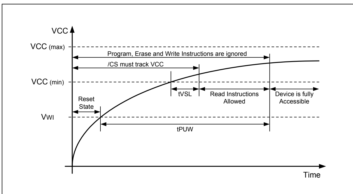
Figure 26. Power-up Timing and Voltage Levels
