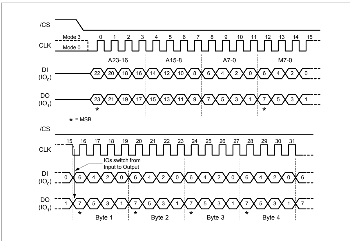
Figure 12b. Fast Read Dual I/O Instruction Sequence (Previous instruction set M5-4 = 10)
