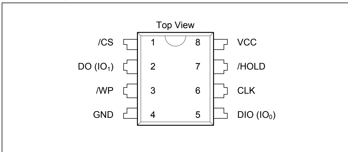
Figure 1c. W25X40BL Pin Assignments, 8-pin PDIP 300-mil (Package Code DA)
