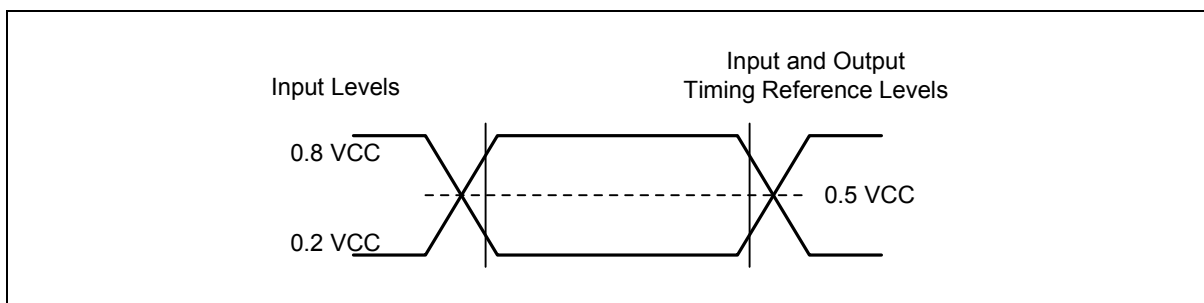
Figure 27. AC Measurement I/O Waveform
