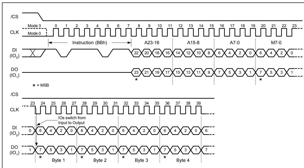
Figure 12a. Fast Read Dual I/O Instruction Sequence (Initial instruction or previous M5-4 ≠ 10)
