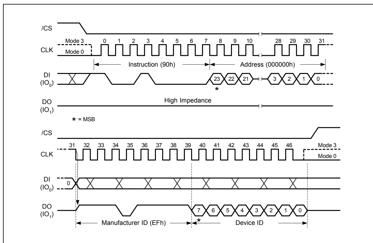
Figure 22. Read Manufacturer / Device ID Diagram
