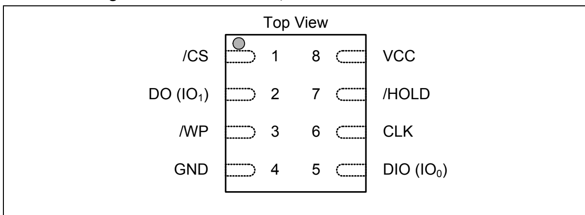
Figure 1b. W25X40BL Pad Assignments, 8-pad WSON 6x5-mm, USON 2x3-mm (Package Code ZP & UX)
