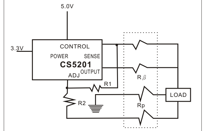
Figure 2. Remote Load Sensing
