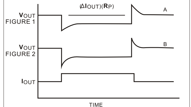
Figure 3. Remote Sensing Improves Load Regulation
