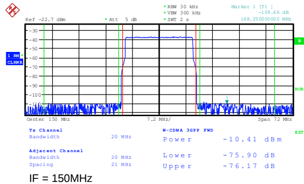
Figure 53. 20MHz Single Carrier LTE Test Mode 3.1
