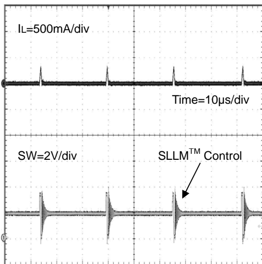
Figure 36. Switching Waveform with SLLM^{TM} ( V_{IN} = 3.3V , V_{OUT} = 1.8V , I_{OUT} = 30mA , L=2.2\mu H )
