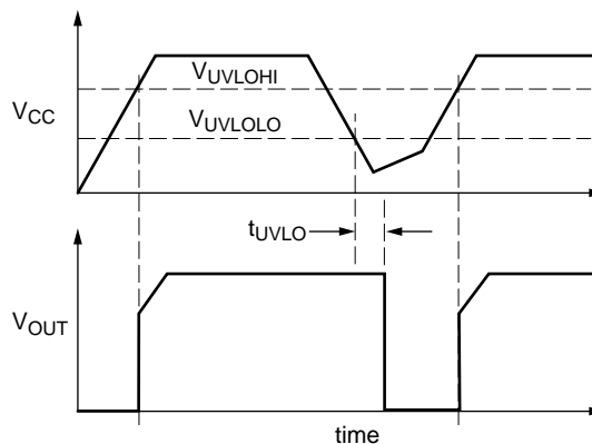
Figure 3. Definition of Undervoltage Lockout
