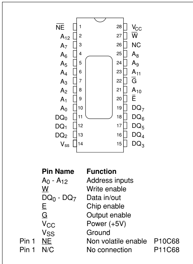
Figure 1. Pin connections - top view.
