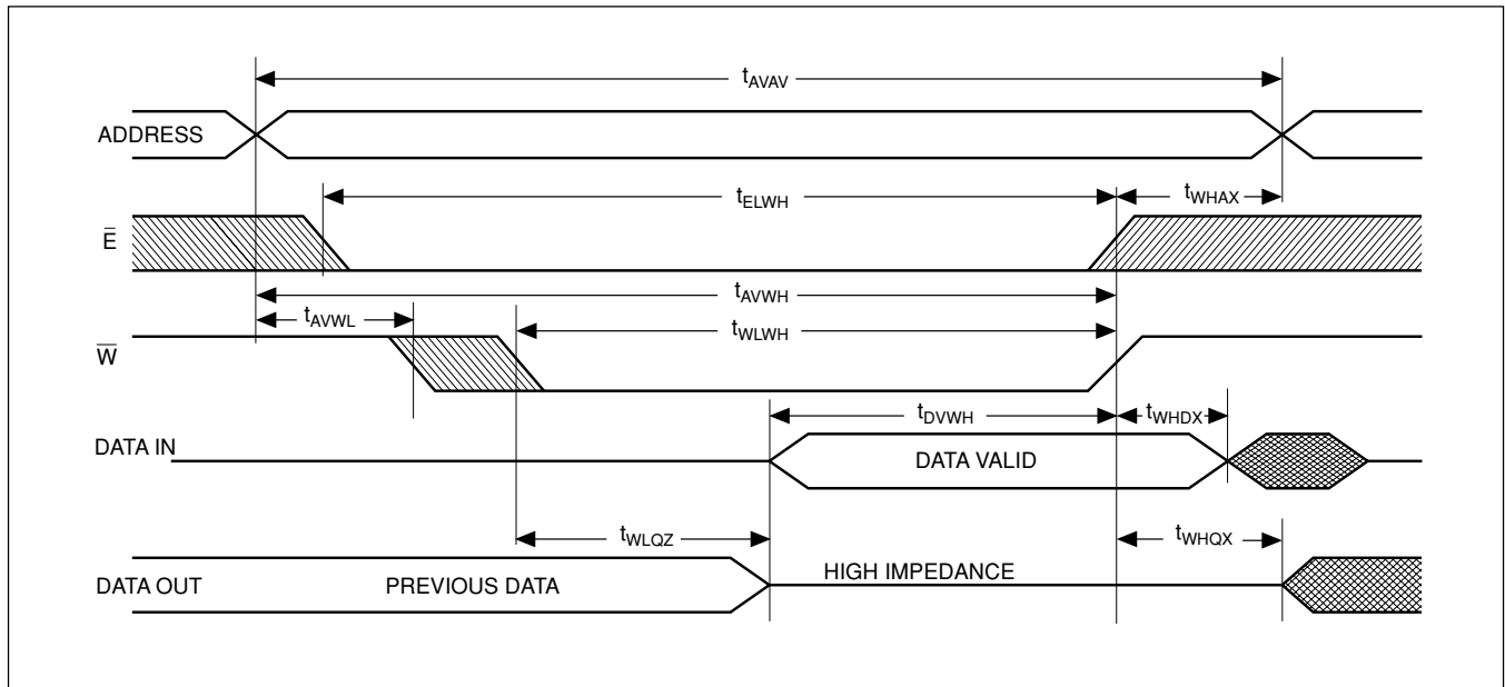
Figure 6. WRITE CYCLE 1: \overline{W} (bar) controlled timing diagram (see notes 8 and 13).
