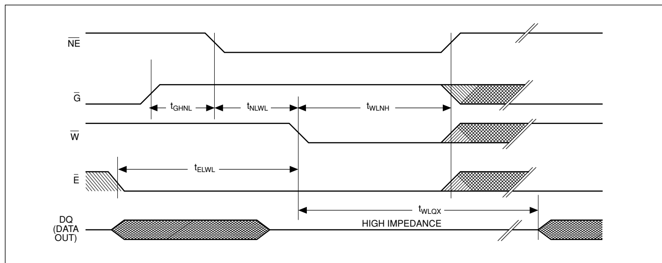
Figure 9. STORE CYCLE 1: W (bar) controlled timing diagram (see note 16).
