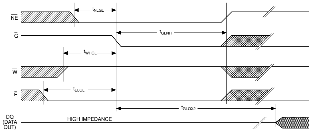
Figure 13. P10C68 RECALL CYCLE 3: E (bar) controlled timing diagram (see note 16).
