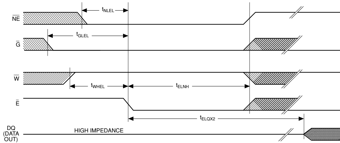
Figure 12. P10C68 RECALL CYCLE 2: E (bar) controlled timing diagram (see note 16).
