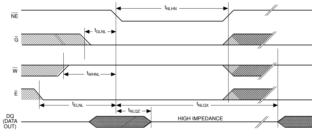
Figure 11. P10C68 RECALL CYCLE 1: NE (bar) controlled timing diagram (see note 16).
