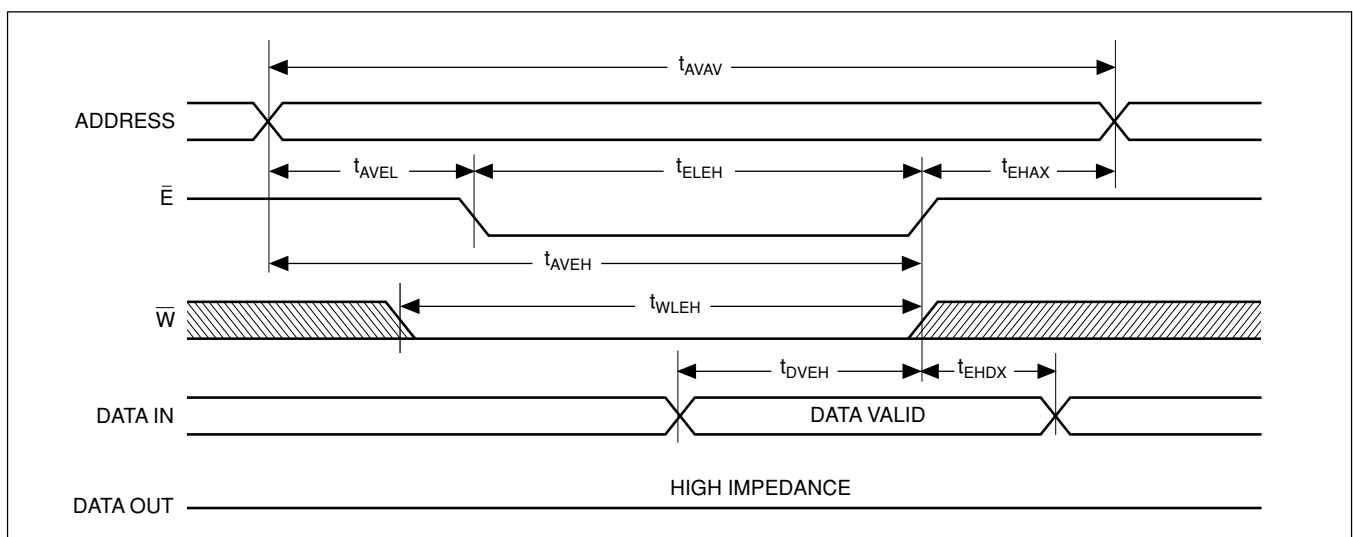
Figure 7. WRITE CYCLE 2: \overline{E} (bar) controlled timing diagram (see notes 8 and 13).
