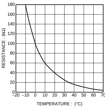
Fig.6 Thermistor curve
