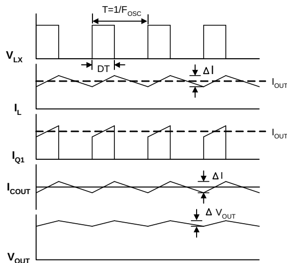
Figure 1. Converter Waveforms
