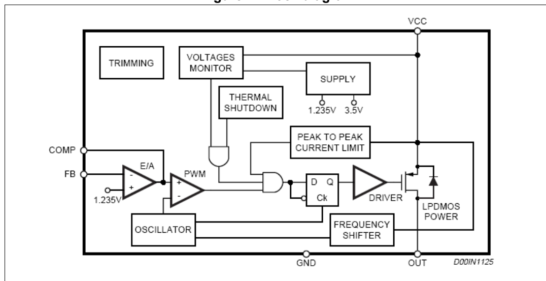
Figure 2. Block diagram
