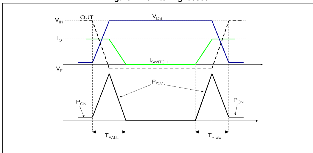
Figure 12. Switching losses
