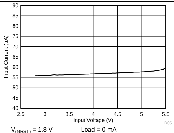
图 7. PFM Mode Current Consumption vs Input Voltage, One Regulator Enabled (1+1+1+1-Phase Output)
