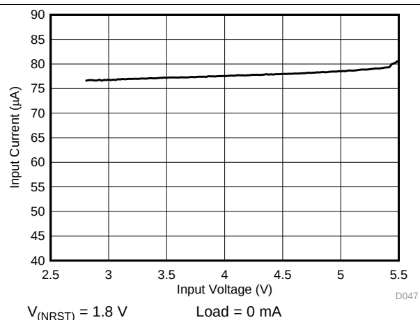
图 4. PFM Mode Current Consumption vs Input Voltage (4-Phase Output)
