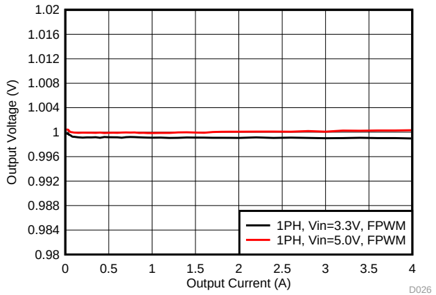
图 49. Output Voltage vs Load Current in Forced-PWM Mode (1-Phase Output)
