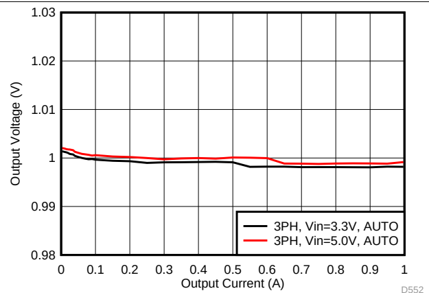
图 51. Output Voltage vs Load Current in PFM/PWM Mode (3-Phase Output)
