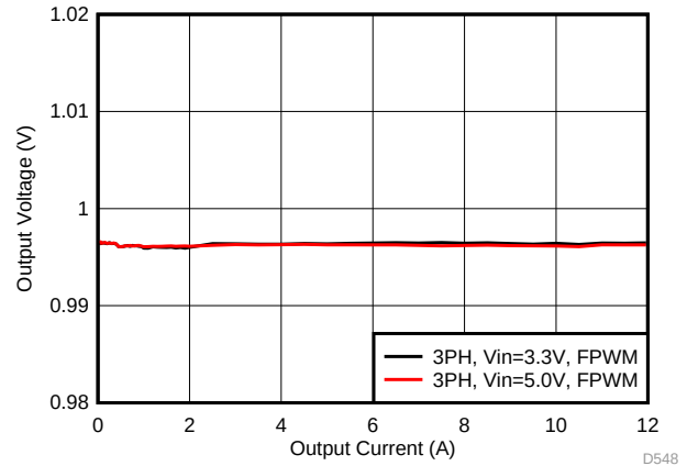
图 47. Output Voltage vs Load Current in Forced-PWM Mode (3-Phase Output)
