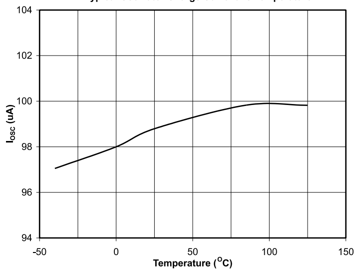
Typical Oscillator Charge Current vs Temperature
