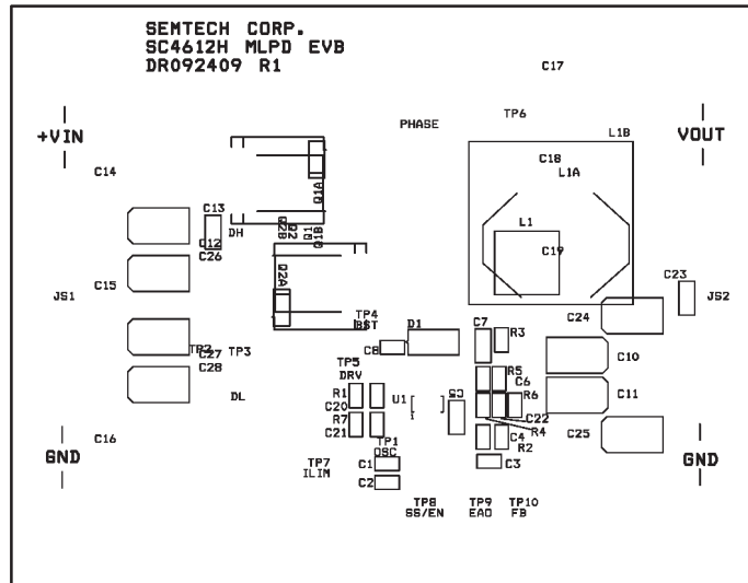
Top Silk Screen
