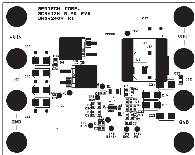
Top Assembly
