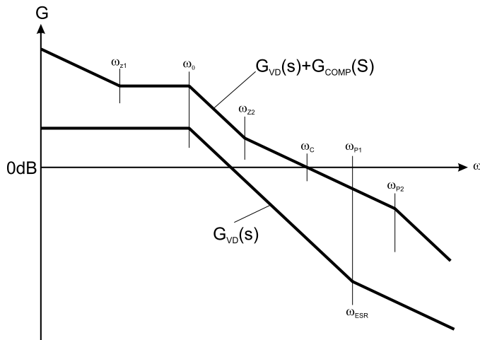
Fig2. Power stage and compensated loop gain.
