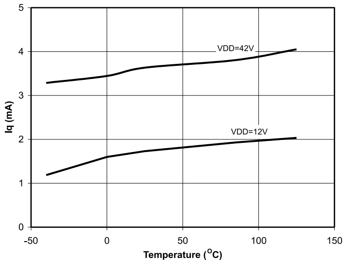
Typical VDD Quiescent current vs Temperature
