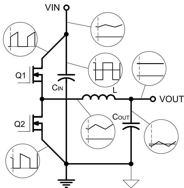
Fig4: Current waveforms of buck power stage.
