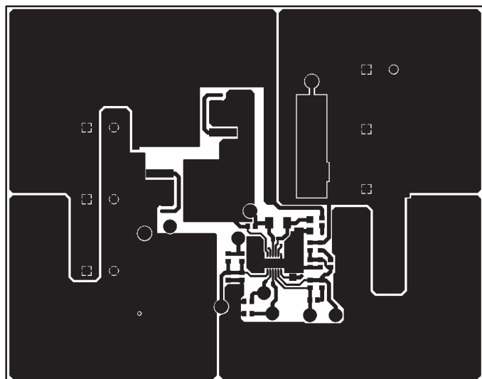
Top Copper
