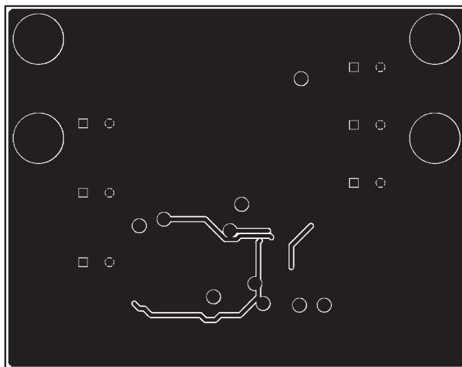
Bottom Copper (viewed from top)
