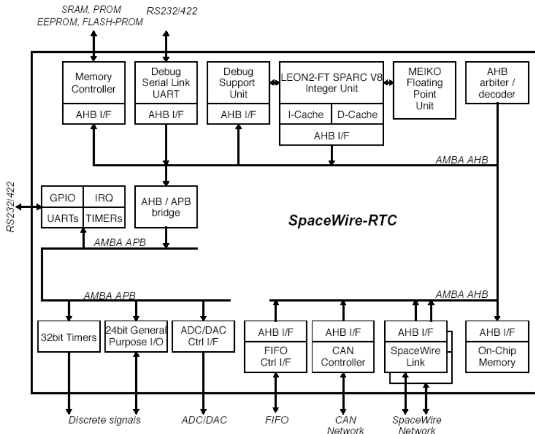
Figure 1-1. AT7913E SpaceWire RTC Block Diagram
